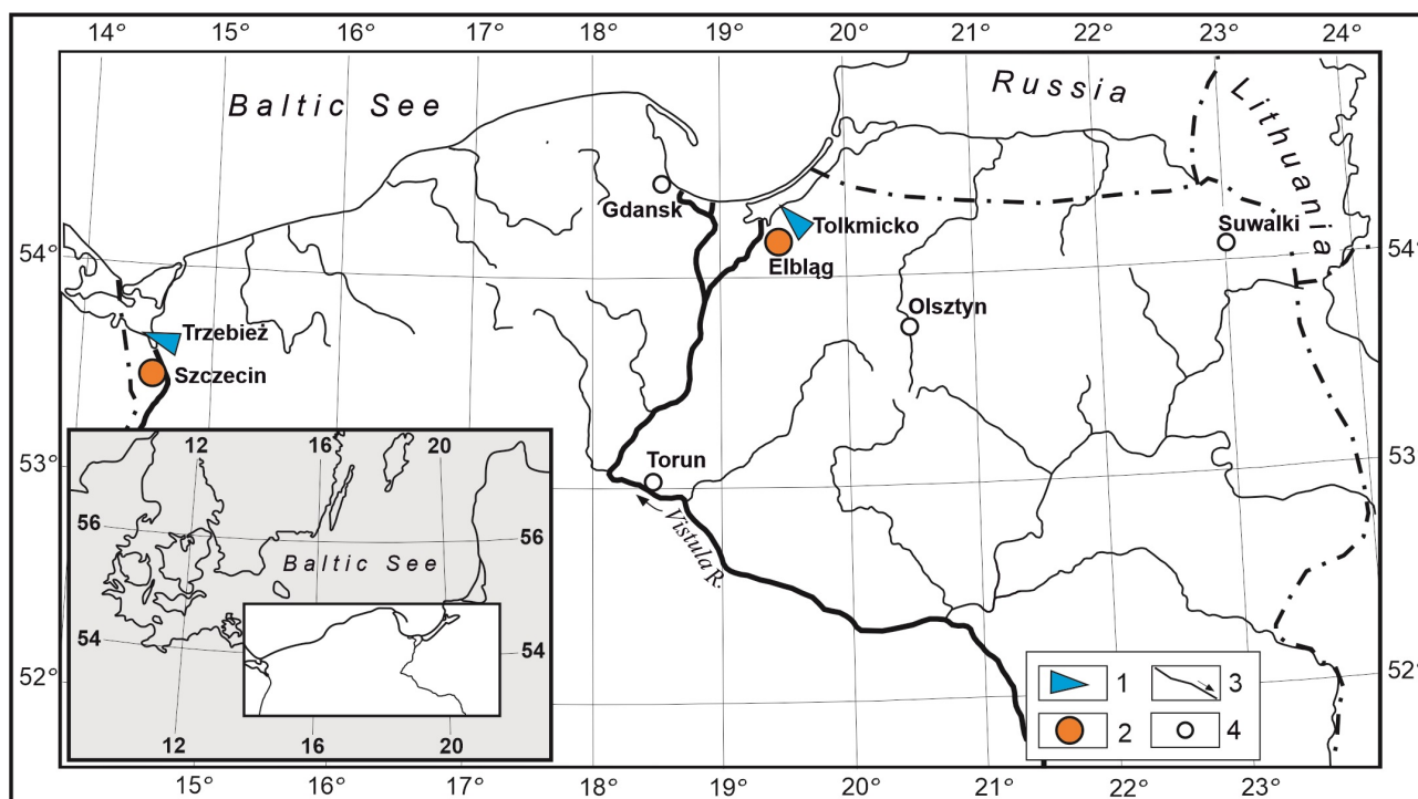
Figure 1. Location of the lagoons of the southern Baltic Sea. 1) Gauging station; 2) Meteorological station; 3) River; 4) City.
