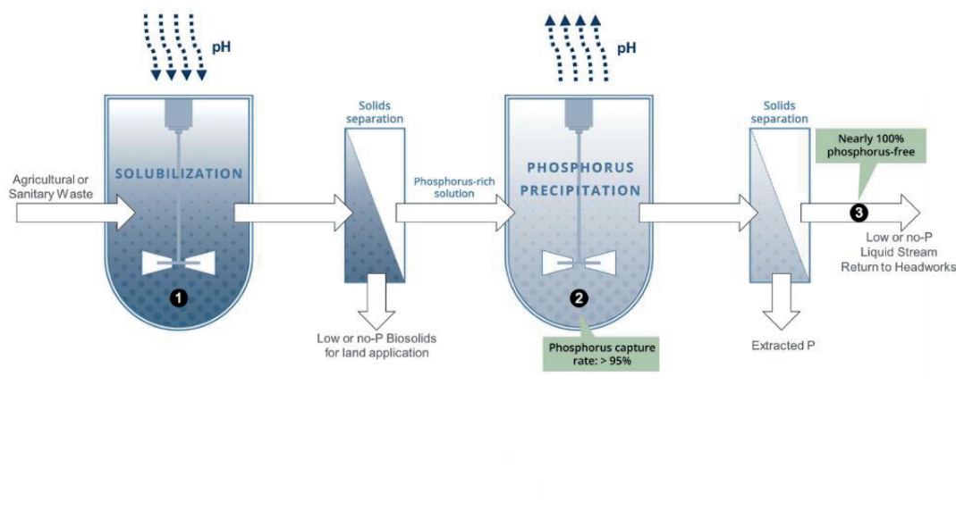
Fig. 2. Schematic diagram of the two-stage Quick Wash ® P recovery process developed by Renewable Nutrients; source: Renewable Nutrients
