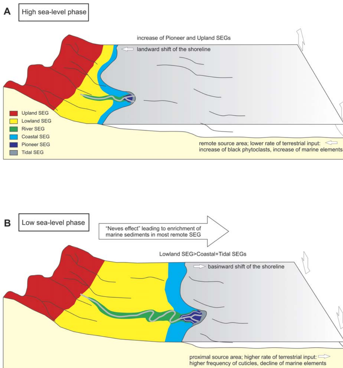
Text-fig. 14. Conceptual reconstruction of the palaeogeography of the Częstochowa area during the Bathonian based on palynofacies and analysis of SEGs. A – high sea-level phase; B – low sea-level phase
