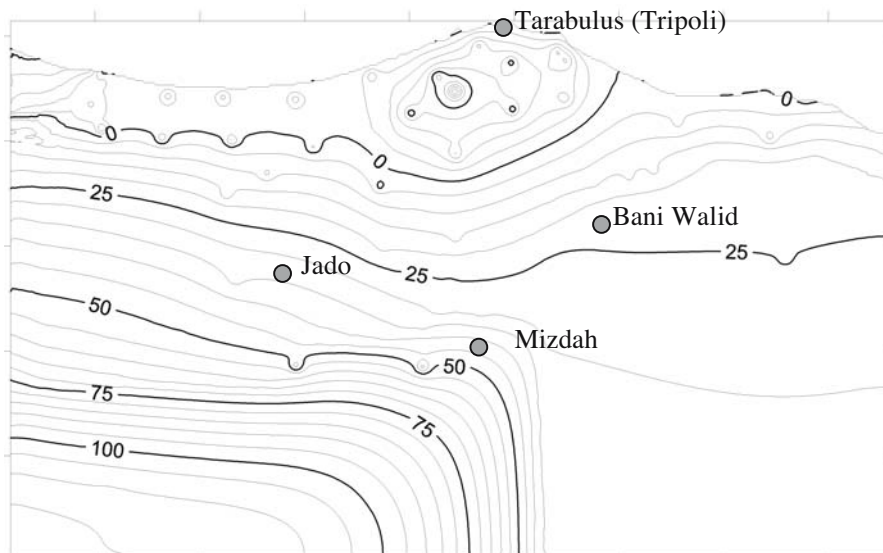
Text-fig. 4. Piezometric surface under natural conditions as a result of the numerical modelling of the whole aquifer system
