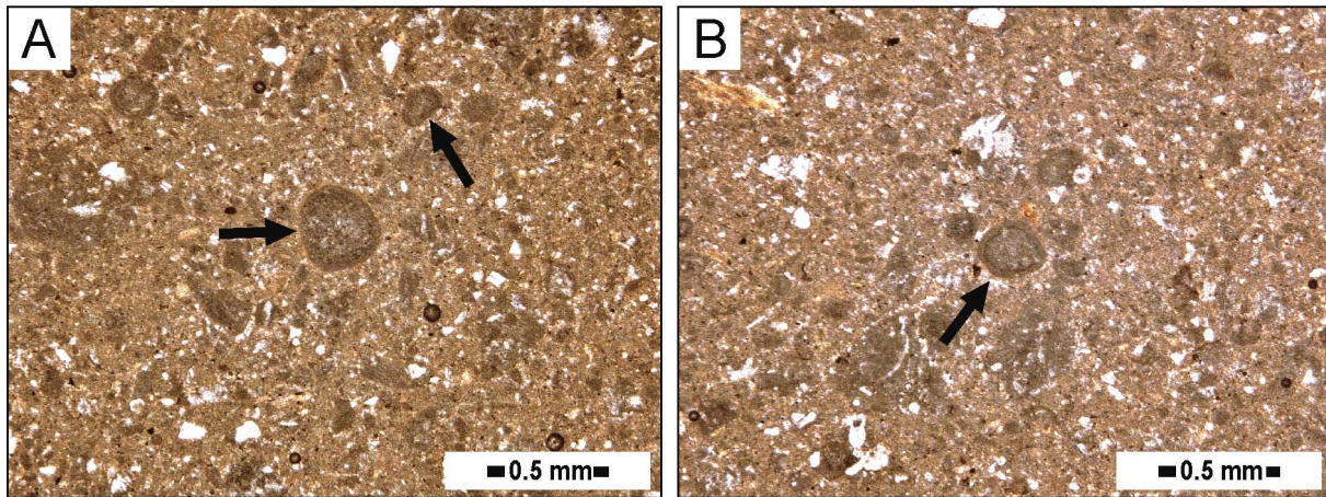
Text-fig. 7. Examples of microscopic images of compacted sample 1 subjected to 336.35 kPa load. Grain size distribution corresponds to wackestones from Upper Jurassic detrital limestones at the Żary quarry (oriented sample, top surface upward). A – tuberooids among coarser grains with common brownish rims (arrows). B – centre: brownish rim (arrow) seen at the bottom surface of microoncooid. Small pores result from washout of sediment during preparation of thin section
