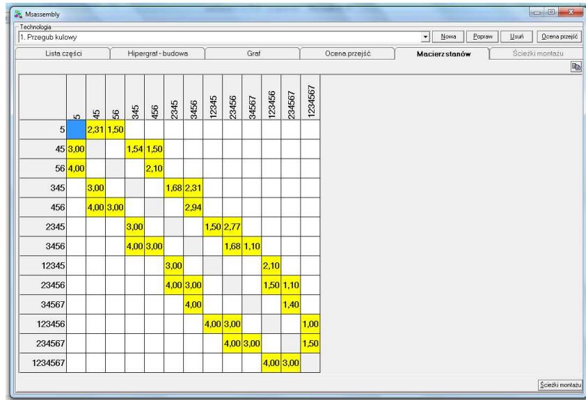
Fig. 3. View of a window of the state matrix in the Mssassembly program
