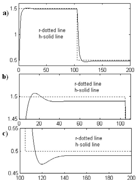
Fig. 5. a) Time responses of the sltank,mdl with fuzzy controller, b) and c) the zoomd responses
