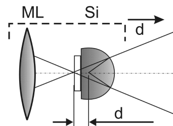
Fig. 19. Position of the setup: ML – microscopy lens, Si – silicon lens, d – displacement of the THz beam focus
