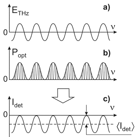
Fig. 17. The idea of coherent homodyne detection. a) E_{THz} – THz ray, b) P_{opt} – detecting beam, c) I_{det} – signal at the receiving chip, \langle I_{det} \rangle – nonzero average signal
