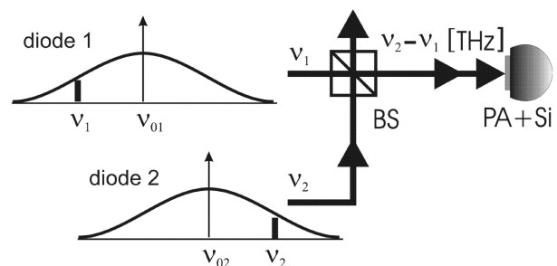
Fig. 2. Illustration for the two laser diode heterodyne operation with slightly moved central frequencies \nu_{01} and \nu_{02}
