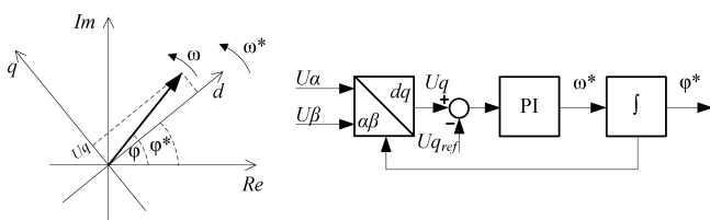
Fig. 3. Concept of Synchronous Reference Frame PLL (SRF-PLL)
