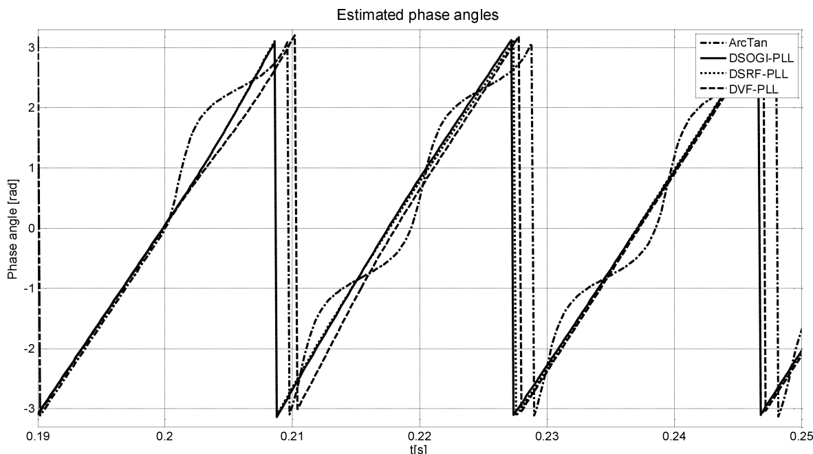
Fig. 12. Estimated phase angle
