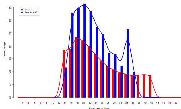
Fig. 4. Domain coverage by alignments found by BLAST and SeedBLAST
