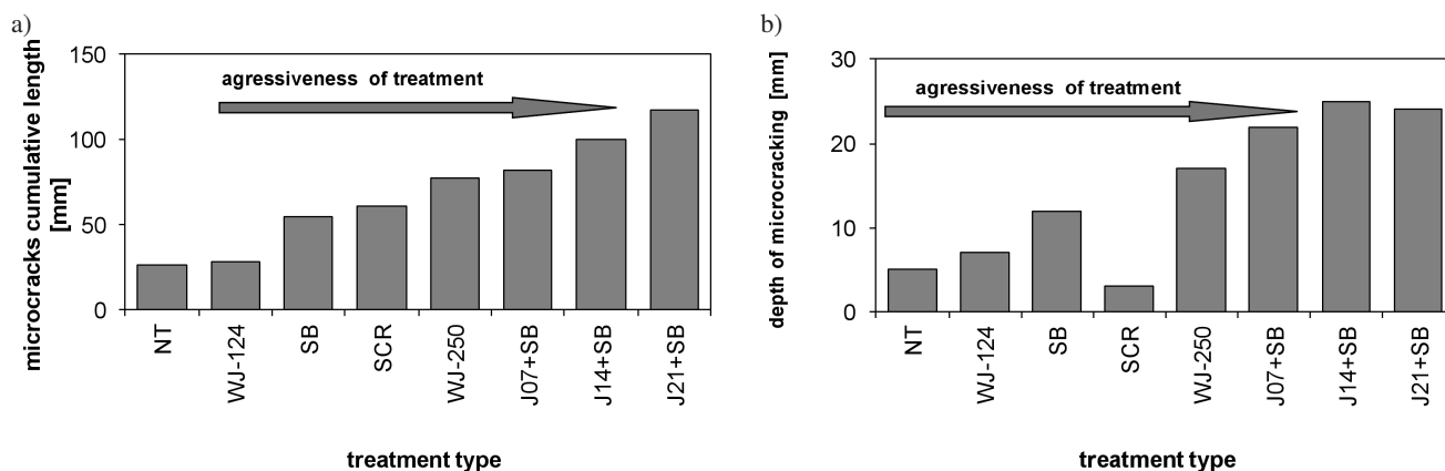
Fig. 11. Length (Li) of the cracks (a) and depth of microcracking (b) vs type of concrete surface treatment: NT – no treatment; WJ – water jetting – pressure 124 psi/250MPa; SB – sandblasting; SCR – scabbling; J+SB – jack hammering of weight 7,14,21 kg + sandblasting after Ref. 10
