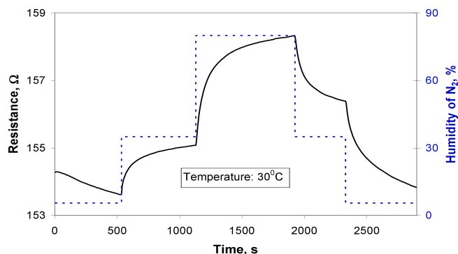
Fig. 8. Response of the structure with palladium layer affected by humid nitrogen; temperature of the structure: 30°C
