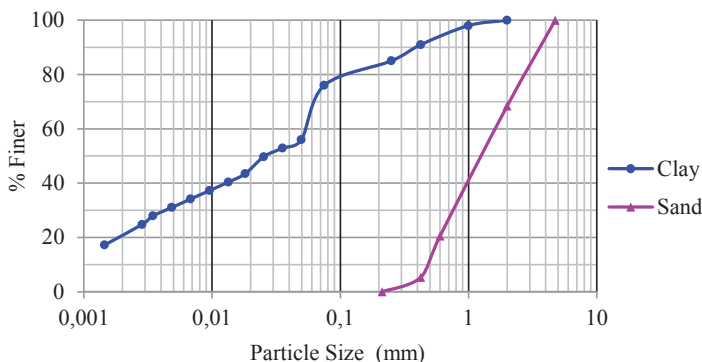
Fig. 2. Particle size distribution of clay and sand.
