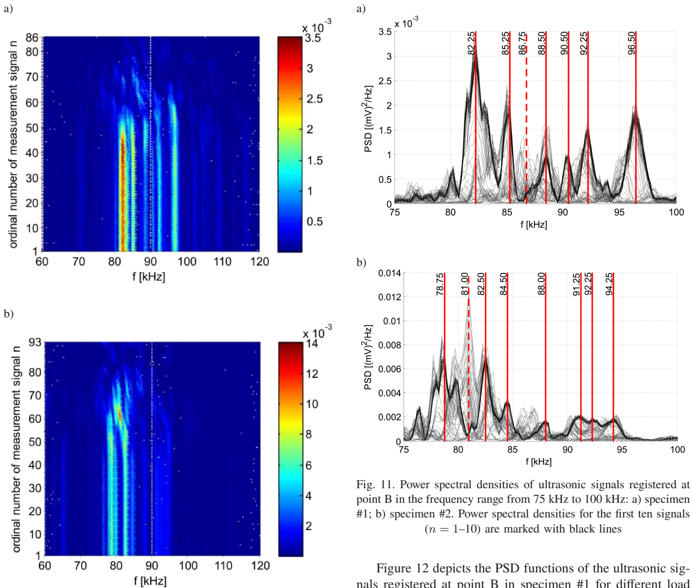
Fig. 10. Power spectral density maps of signals registered at point B: a) specimen #1; b) specimen #2 (power spectral densities are in units of (mV)^2/Hz )
