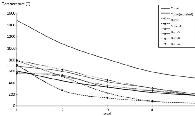
Fig. 3. Measured and calculated center-line temperature distribution for Burns 1-8. Burn 1,2,5,8 (through-draft conditions), Burn 3,4,7 (no-through-draft conditions) Ref. 7
