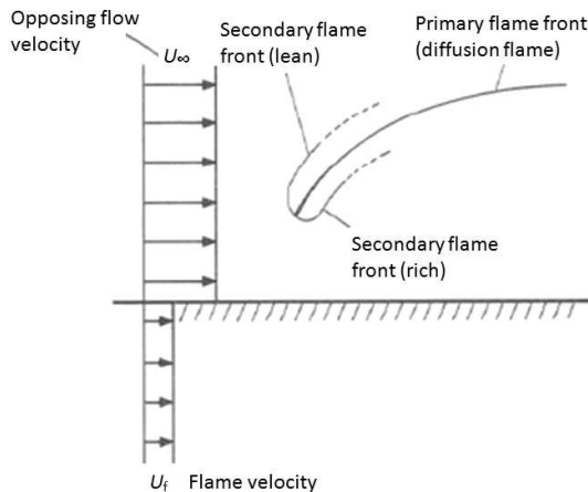
Fig. 6. The flame spread model by deRis (Ref. 23)
