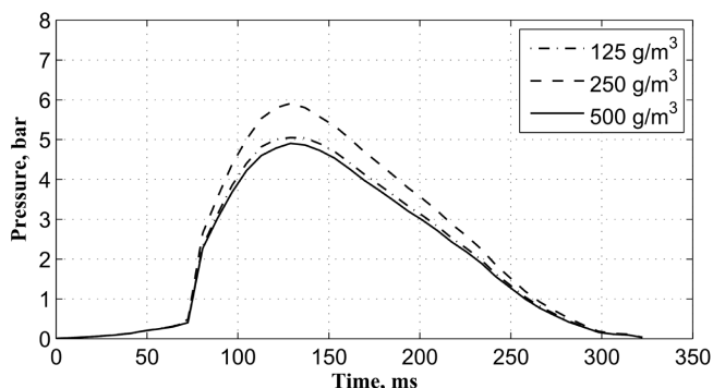
Fig. 8. Pressure changes for the simulation of coal dust explosion
