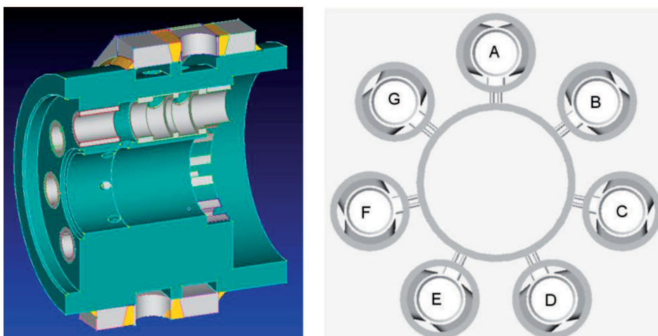
Fig. 7. Cross section through the pump body showing half of the pump body without pistons (left) and the location of all 7 pressure chambers around the perimeter of the compensation chamber (right)
