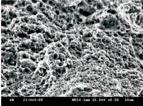
i) T_A=800^\circ\text{C} + T_T=675^\circ\text{C}
