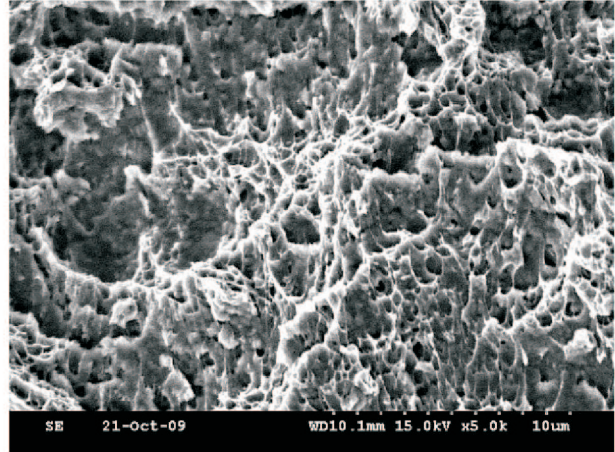
h) T_A=800^\circ\text{C} + T_T=650^\circ\text{C}
