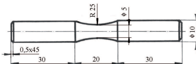
Fig. 1. Specimen shape used in the present investigation
