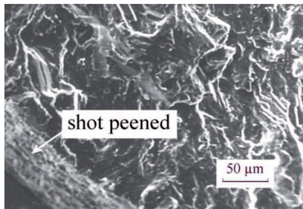
Fig. 3. Fatigue fracture of the specimen with shot peened surface with thickness of approx. 50 \mu m
