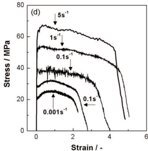
Fig. 1d Stress-strain curves at temperature of 723 K
