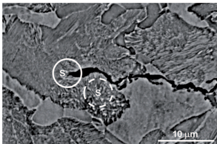
Fig. 4. A crack observed in the forging ingot as the result of increased amount of the sulphur, denoted as the S – areas, [5]
