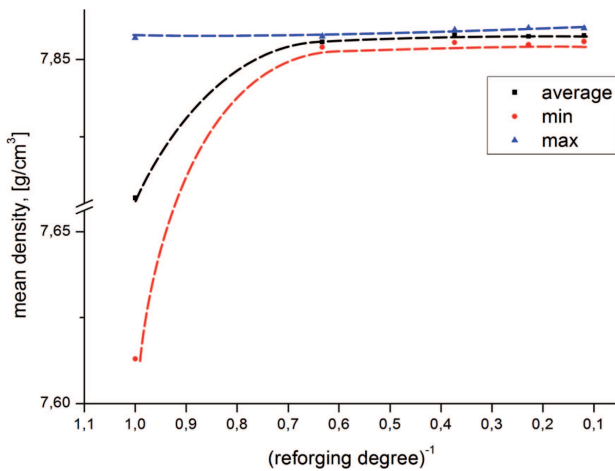
Fig. 25. Comparison of the local densities after applied re-forming degree
