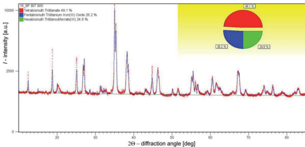
Fig. 7. X-ray diffraction patterns of 16%(BF-BiT)//BiT composite
