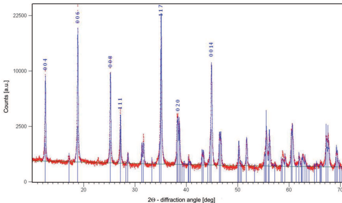
Fig. 4. X-ray diffraction pattern of \text{Bi}_4\text{Ti}_3\text{O}_{12} ceramic powder at room temperature
