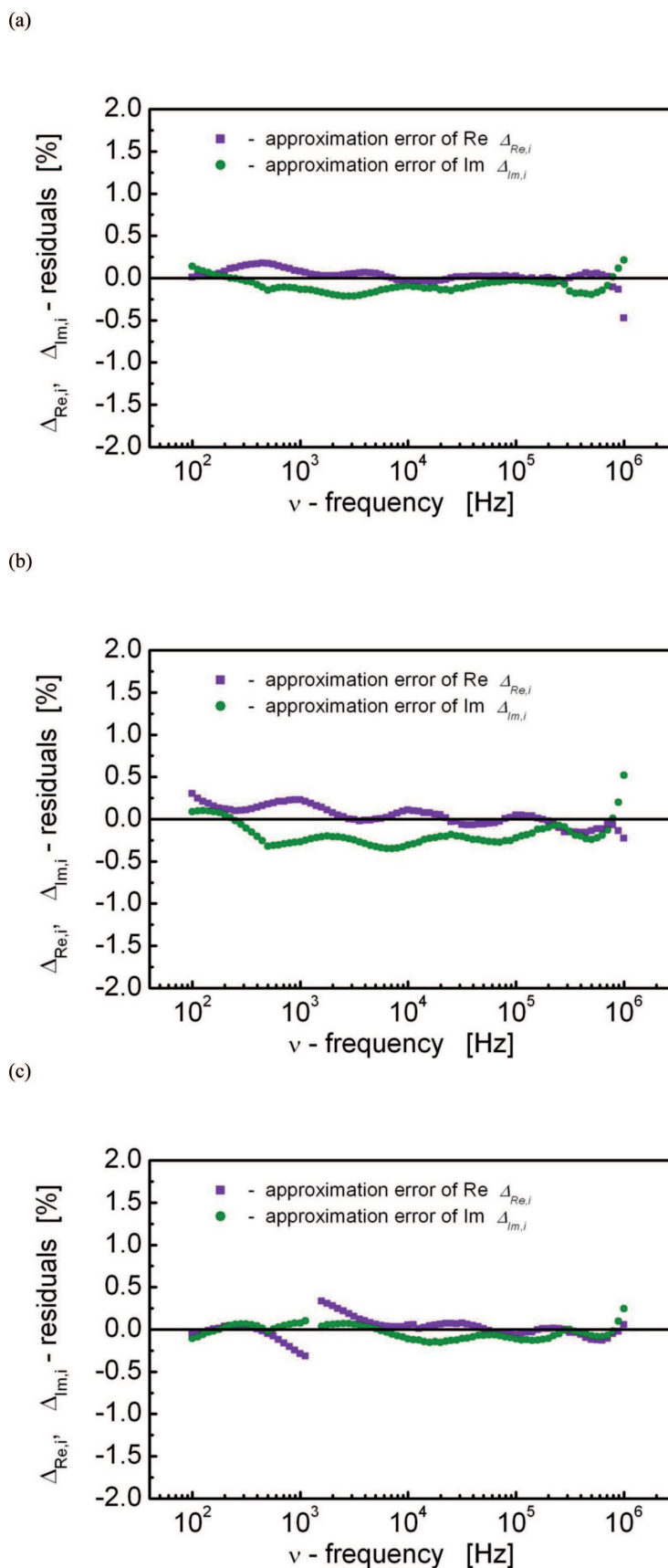
Fig. 8. FQ-plots for the final parameter set obtained with the dispersion analysis program for \text{Bi}_4\text{Ti}_3\text{O}_{12} ceramics at temperature range \Delta T=200\text{--}500^\circ\text{C} ( T=200^\circ\text{C} (a), T=400^\circ\text{C} (b), T=500^\circ\text{C} (c))
