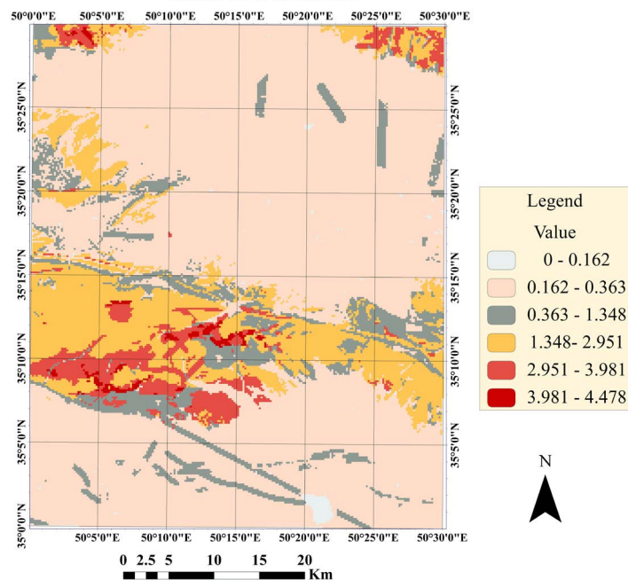
Fig. 8. Exploration priority map of C-A fractal modeling of integrated information layers in Saveh 1:100,000 sheet
