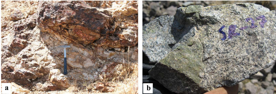
Fig. 5. a) Argillic alteration with iron hydroxide impregnation resulted from disintegration of pyrite grains, b) macroscopic sample of gabbro-diorite with epidotized xenolith as an indicator of propylitic alteration in Saveh 1:100,000 sheet
