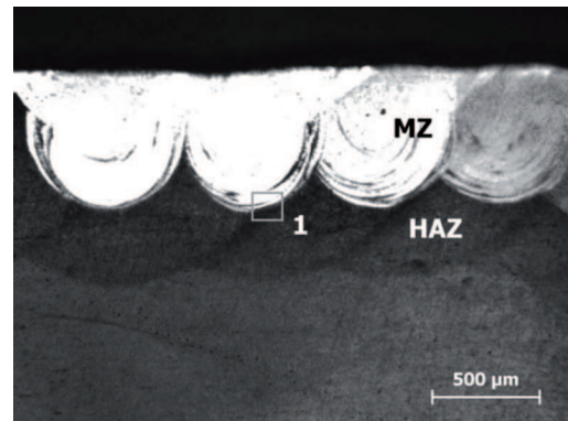
Fig. 1. Microstructure of C45 steel after borochromizing and LHT q = 41.40 \text{ kW/cm}^2 , v = 0.67 \text{ m/min} ; Reagent: solution 2% HNO 3
