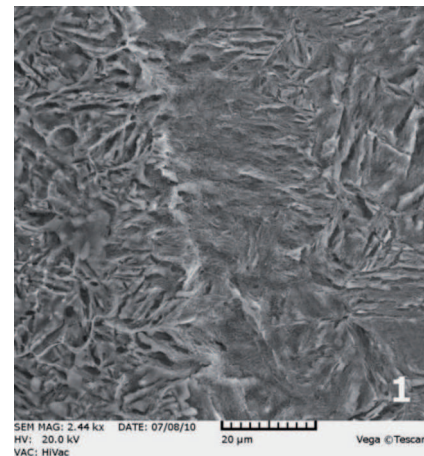
Fig. 2. Microstructure of C45 steel after borochromizing and LHT q = 41.40 \text{ kW/cm}^2 , v = 0.67 \text{ m/min} ; boundary MZ and HAZ; Reagent: solution CuSO 4 + HCl + H 2 O
