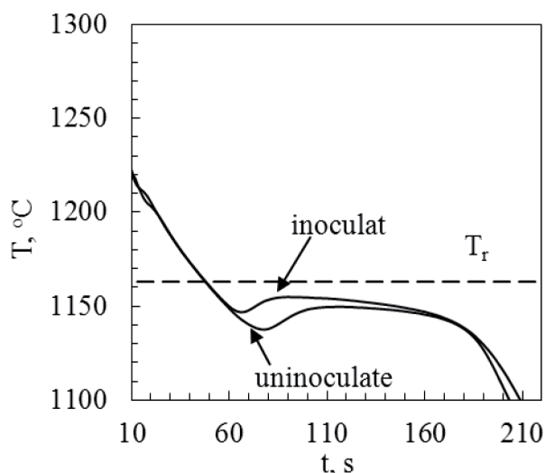
Fig. 11. Cooling curve of cast irons
