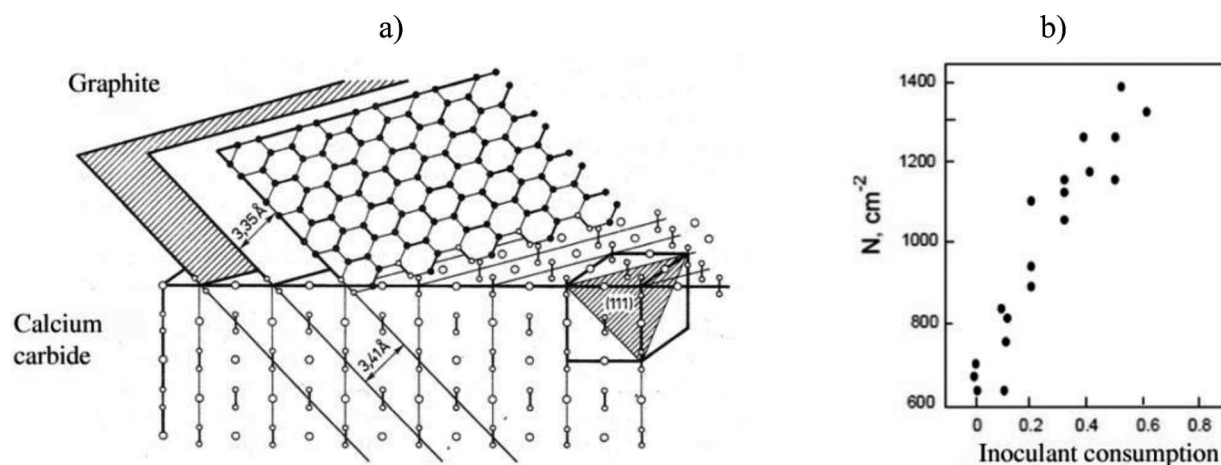
Fig. 17. Similarity of lattice parameters of graphite and calcium carbide (a) and influence of inoculant consumption (ferrosilicon with calcium additions) on cell count of graphite eutectic (b)
