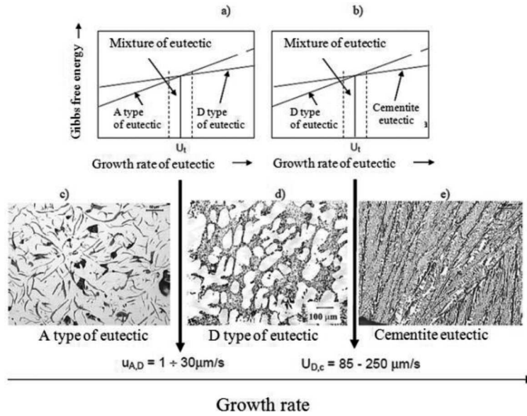
Fig. 7. Influence of growth rate on free energy of eutectics (a,b); u_{A,D} – trasformation rate of A to D type of eutectic, u_{D,C} - trasformation rate of D type to cementite eutectic, microstructures (c,d,e) of A, D and cementite eutectics, respectively; values of transformation rates deal with pure Fe-C alloys
