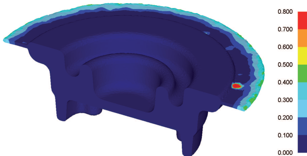
Fig. 7. Distribution of damage criterion (according to Cockcroft-Latham) in a rim forging in the hammer forging process in final impression
