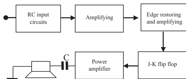
Fig. 4. Block diagram of PAN receiver wiring.
