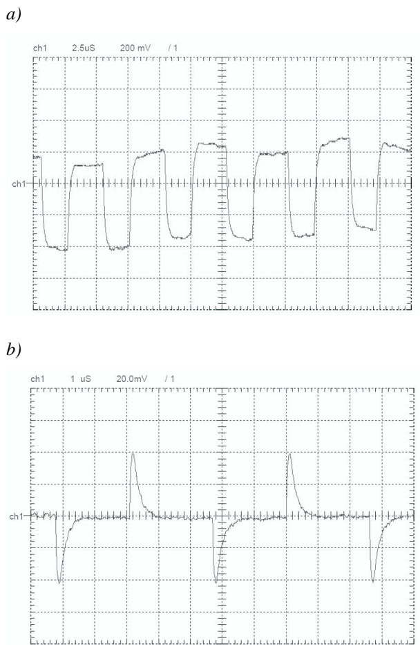
Fig. 3. Curve of the PWM signal, a) without the RC element b) RC element C=82 \text{ pF} , R=1 \text{ k}\Omega .
