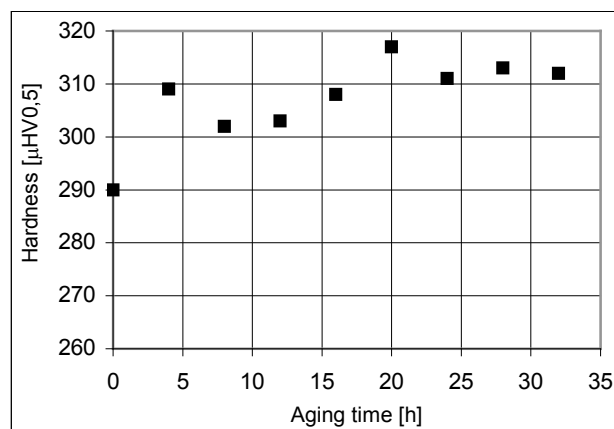
Fig. 2. The Vickers hardness as a function of aging time at a temperature 300°C
