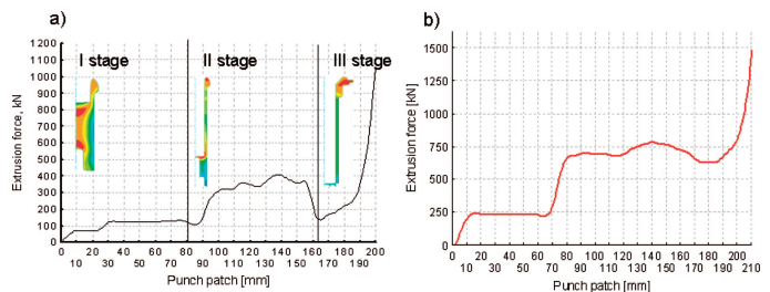
Fig. 4. The diagrams of the relationship of extrusion force versus ram path: a) double-side complex extrusion; b) indirect extrusion
