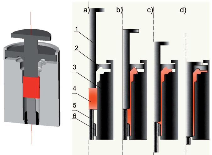
Fig. 2. The tool model and the method for double-sided extrusion a) stage I, b) stage II, c) stage III, d) finished product [8] 1. upper punch with pressure plate, 2. die forging, 3. container, 4. perform, 5. bottom punch, 6. ring
