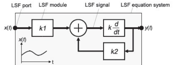
Fig. 2. A LSF model with 4 LSF modules [4].
