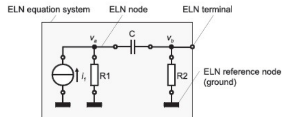
Fig. 3. A basic ELN model [4].
