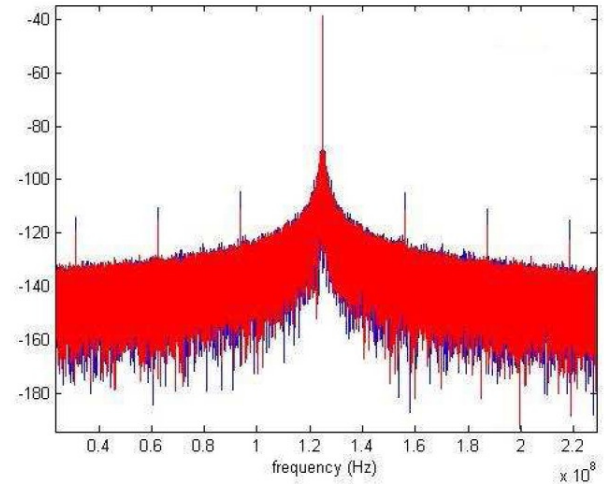
Fig. 10. PSD of VCO output of our and Matlab models.
