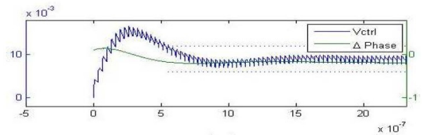
Fig. 11. VCO control voltage of the Matlab model.
