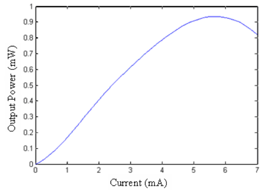
Fig. 2. Output power vs. current for 2\mu\text{m} single mode VCSEL.
