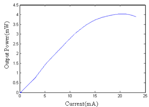
Fig. 3. Output power for 10\mu\text{m} multi mode VCSEL.
