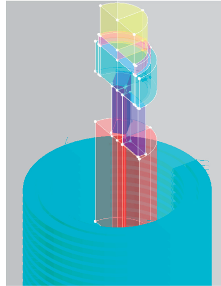
Fig. 7. Calculation model
