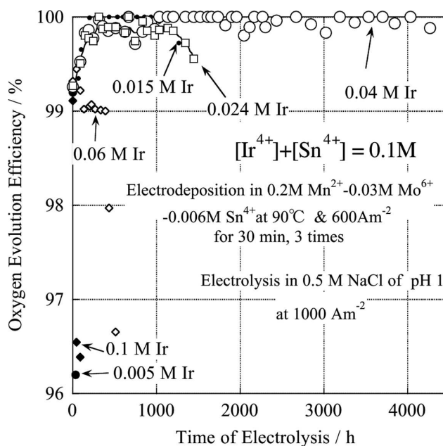
Fig. 7. Dependence of oxygen evolution efficiency at current density of 1000 \text{ Am}^{-2} in 0.5 \text{ M NaCl} solution at pH 1 on duration of electrolysis for the anodes consisting of \text{Mn}_{1-x}\text{Mo}_x\text{Sn}_y\text{O}_{2+x} electrocatalyst prepared by anodic deposition for 30 min, 3 times over \text{IrO}_2 and \text{Sn}_{1-x}\text{Ir}_x\text{O}_2 intermediate layers [13]. Intermediate \text{IrO}_2 layer was prepared from 0.1 \text{ M H}_2\text{IrCl}_6 butanol solution, and \text{Sn}_{1-x}\text{Ir}_x\text{O}_2 layers were prepared from butanol solutions in which the sum of \text{H}_2\text{IrCl}_6 and \text{SnCl}_4 was 0.1 \text{ M}
