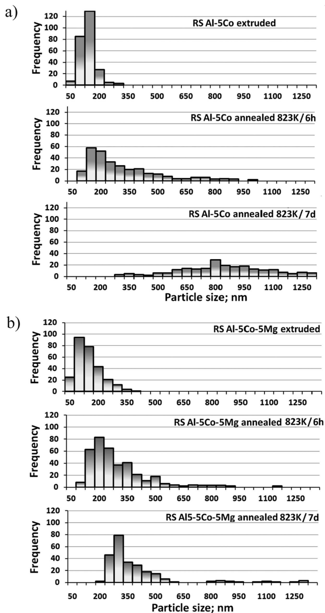
Fig. 10. Distribution of \text{Al}_2\text{O}_3 particles in as-extruded and annealed RS alloys (a) Al-5Co; (b) Al-5Co-5Mg. Heat treatment conditions (823K/6h, 823K/168h) are marked in the figure
