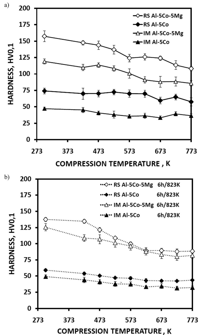
Fig. 3. Hardness of samples deformed by compression ( \epsilon_c \approx 0.4 ) vs. deformation temperature: (a) as-extruded RS and IM materials; (b) RS and IM samples preliminarily annealed at 823K/6h. Tested materials are listed in a legend
