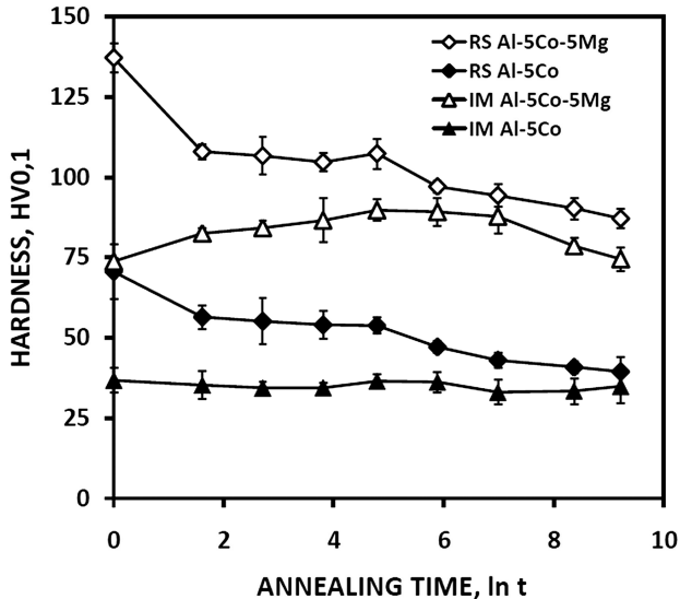
Fig. 4. Hardness vs. annealing time curves received for IM and RS Al-5Co and Al-5Co-5Mg alloys annealed at 823 K
