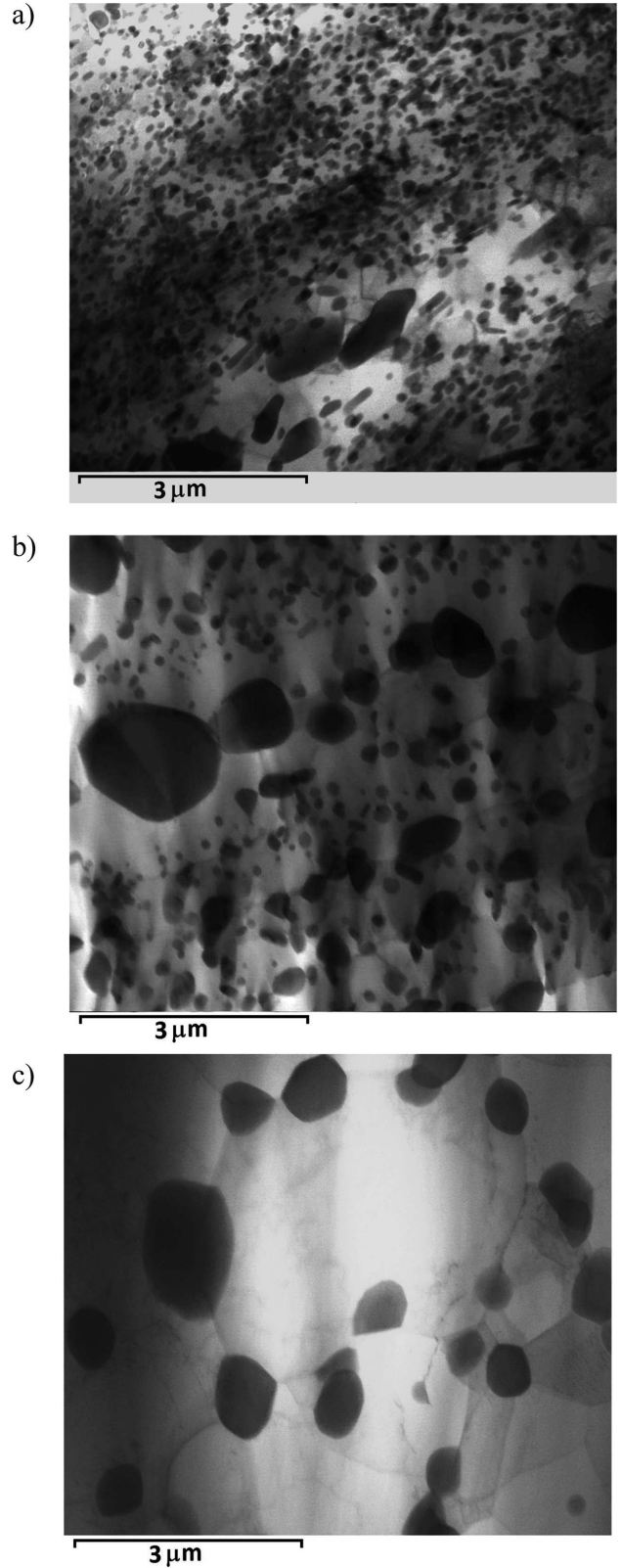
Fig. 8. STEM Structure RS Al-5Co alloy (a) as-extruded (b) annealed 6h/823K (c)annealed 7d/823K
