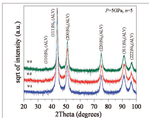
Fig. 4. XRD for the samples V-1, V-2 and V-3 after intensive deformation with HPT. The L1 2 structure of Ni 3 Al phase is seldom present
