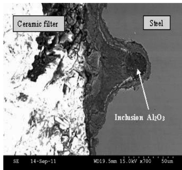
Fig. 10. Scanning pictures of interface partition filters ceramic – filtration steel of head – SE03 steel
