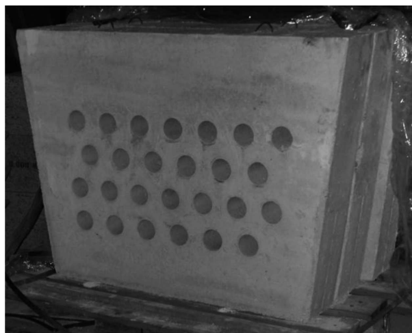
Fig. 4. Multi- hole ceramic filter
