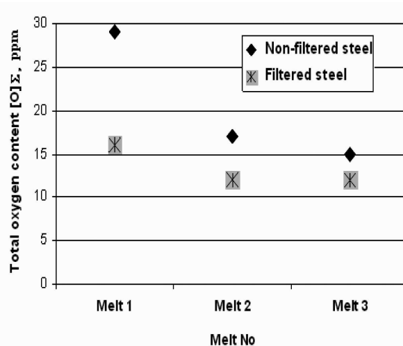
Fig. 5. [O] T total oxygen content variation in each of the melt sequence (second trial) – 34GJ steel
