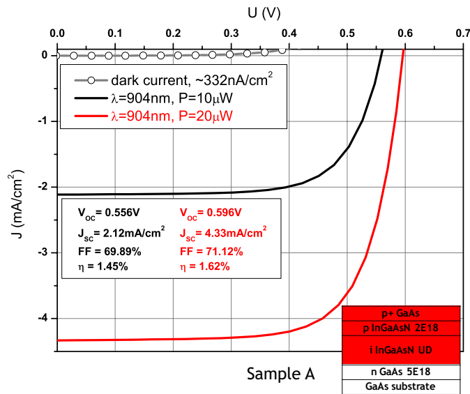
Fig. 7. J-V characteristics of the test solar cell (sample A) measured under an optical excitation of laser diode emitting radiation of \lambda=904 \text{ nm} and optical power of 10 (black curve) and 20 \mu\text{W} (red curve).
