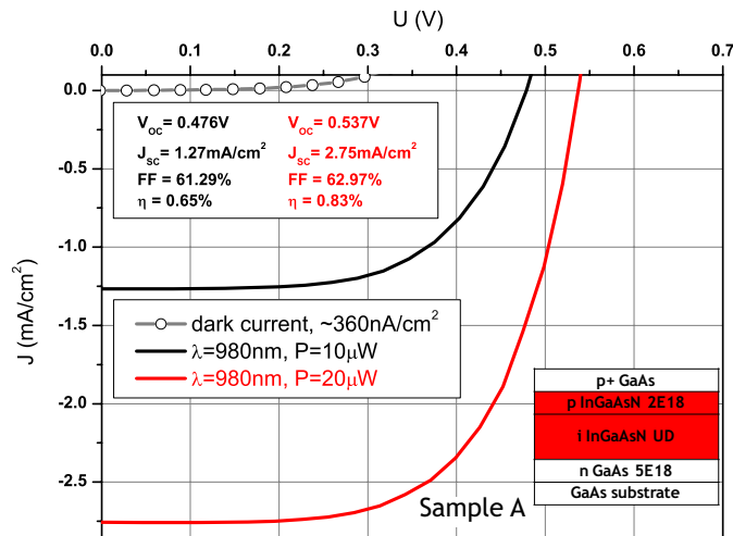
Fig. 8. J-V characteristics of the test solar cell (sample A) measured under an optical excitation of laser diode emitting radiation of \lambda=980 \text{ nm} and optical power of 10 (black curve) and 20 \mu\text{W} (red curve).
