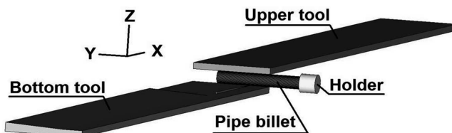
Fig. 3. Geometrical model of the process of splitting the billet pipe used in the FEM analysis
