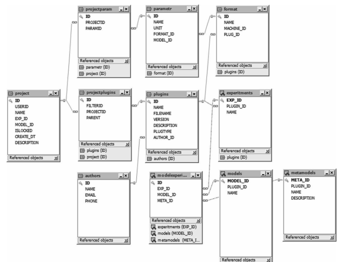
Fig. 3. Database diagram of the proposed computer system
