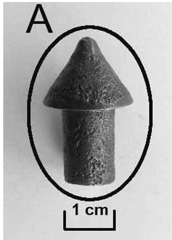
Fig. 12. Investment cast tooth from a working part of the holder
