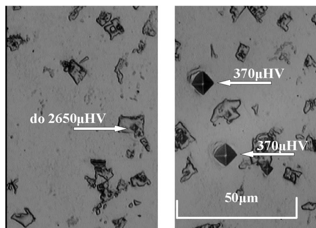
Fig. 6. As-cast microstructure of steel containing 1.65% C and 5.5% V, unetched section (sample L160G10V6, Table 1)
