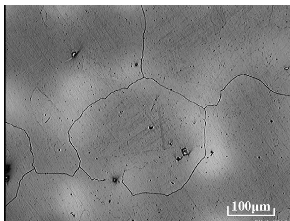
Fig. 5. Cast Hadfield steel after solution heat treatment in water; austenitic matrix free from the precipitates of alloyed cementite at grain boundaries; Nital etching
