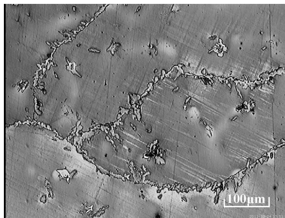
Fig. 4. Hadfield steel in as-cast condition; austenitic matrix with precipitates of acicular alloyed cementite; nital etching
