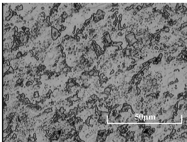
Fig. 7. As-cast microstructure of steel containing 1.65% C and 5.5% V, nital etched (sample L160G10V6, Table 1)
