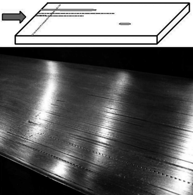
Fig. 1. Preview from the crystallizer's desks defects catalogue [4]
