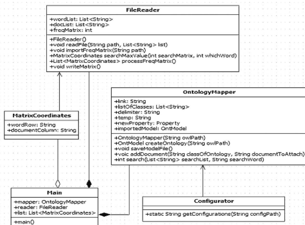
Fig. 2. Fragment of a class diagram
