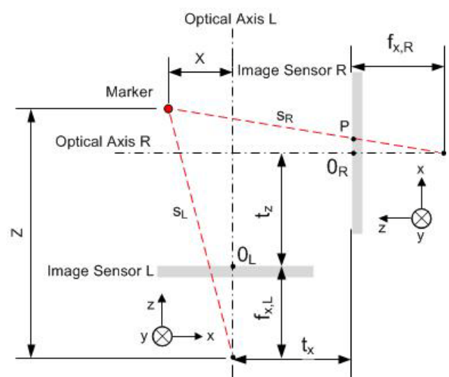
Fig. 8. Geometric Model: Convergent (orthogonal) stereo vision configuration - top view
