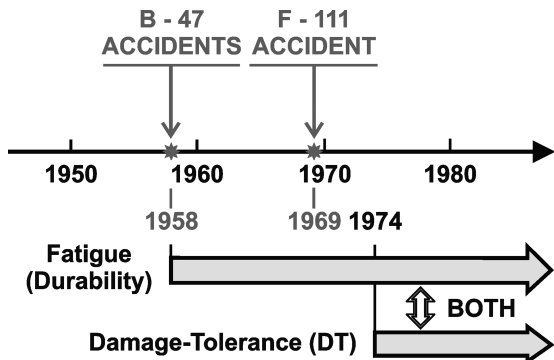
Fig. 1. Key events leading to the adoption of damage tolerance requirements by USAF: (F-111). A full-scale fatigue test of the wing box indicated 16 000 flight hours, a safe life of 6000 hours, whereas the total time in service at the time of the accident was 100 hours. The failure was attributed to a defect which had arisen during the manufacture of the forgings from which the plane was fabricated. The anomalous fatigue resulted in wing separation. Based on [1]
