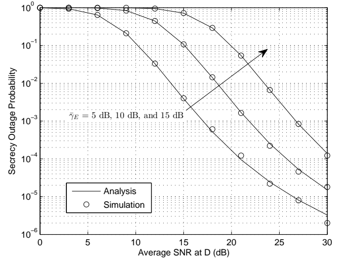
Fig. 3. Secrecy outage probability versus average SNR at destination with R_s = 0.5 bits/s/Hz, K_0 = K_1 = K_2 = 10 , \Gamma/P_s = 9 dB, and \bar{\gamma}_P = 20 dB.
