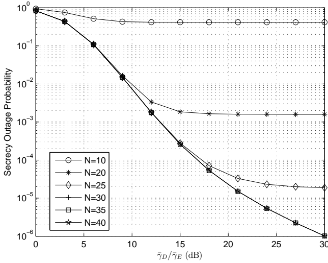
Fig. 2. Secrecy outage probability versus \bar{\gamma}_D/\bar{\gamma}_E with R_s = 0.5 bits/s/Hz, K_1 = 5 , K_0 = K_2 = 10 , \Gamma/P_s = 9 dB, and \bar{\gamma}_P = 20 dB.
