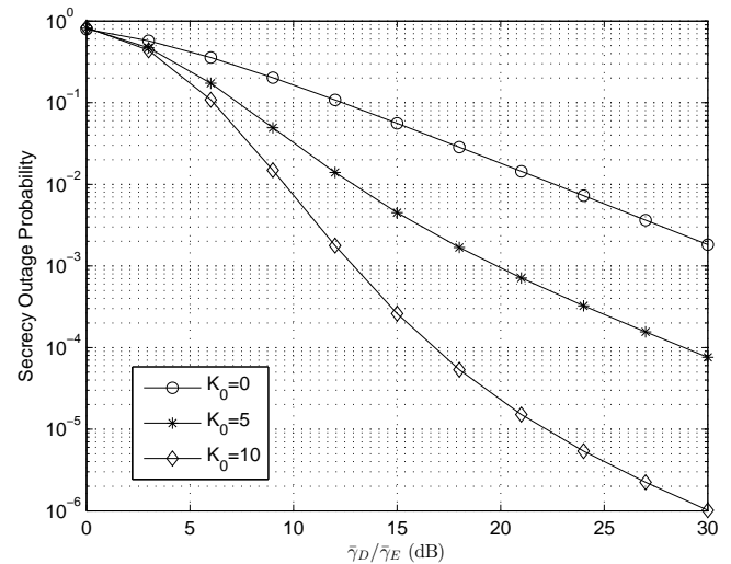
Fig. 4. Secrecy outage probability versus \bar{\gamma}_D/\bar{\gamma}_E with R_s = 0.5 bits/s/Hz, K_1 = 5 , K_2 = 10 , \Gamma/P_s = 9 dB, and \bar{\gamma}_P = 20 dB.
