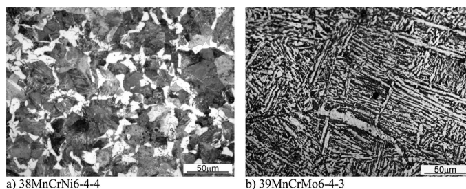
Fig. 1. The microstructures of hypoeutectoid steels in after forging state
