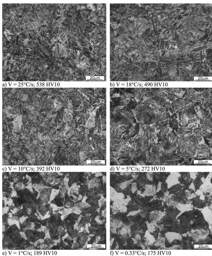
Fig. 7. Microstructures of dilatometric samples used for drawing of CCT diagrams of tested 38MnCrNi6-4-4 steel, austenitized at temperature T_A = 830^\circ\text{C} [14]
