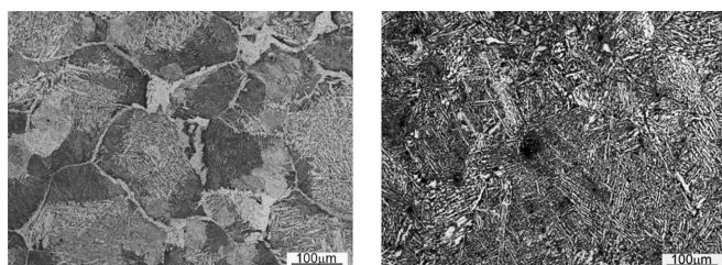
Fig. 2. Microstructures of hypoeutectoid steels after full annealing
