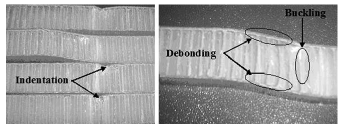
Fig. 6. Various types of skin and core failures
