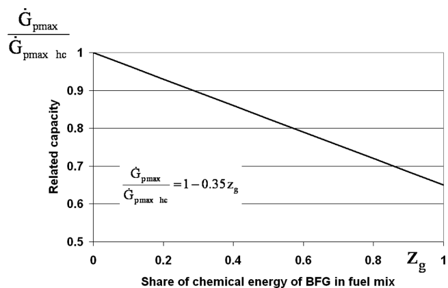
Fig. 1. Capacity of double-fuel boiler vs. share of chemical energy of BFG; \dot{G}_{pmax} – maximum capacity of the boiler fired with fuel mix, \dot{G}_{pmax hc} – maximum capacity of the boiler fired with hard coal
