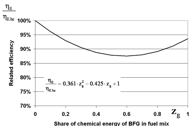
Fig. 2. Efficiency of double-fuel boiler vs. share of chemical energy of BFG; \eta_E – energy efficiency of the boiler fired with fuel mix, \eta_{E hc} – energy efficiency of the boiler fired with hard coal
