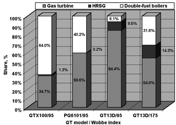
Fig. 15. Shares in utilisation of technological fuel gases
