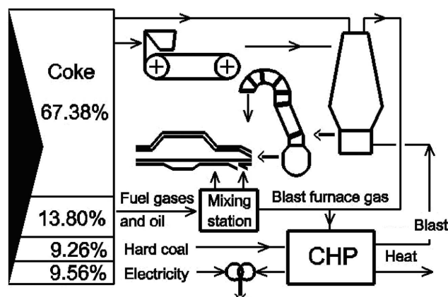
Fig. 3. Structure of energy in ironworks
