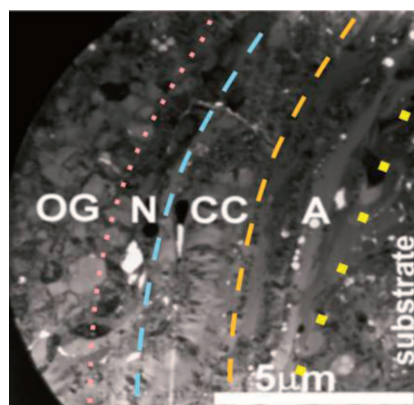
Fig. 13. A separated area which corresponds to the single Fe-Al particle deposited by the D-gun spraying; OG = non-melted part of a particle, N = a typically non-equilibrium \epsilon_N - phase sub-layer, CC = columnar structure of the periodically situated inter-metallic phases ( \text{FeAl} + \text{Fe}_2\text{Al}_5 ) due to the oscillatory mode of solidification, A = \epsilon_A amorphous phase sub-layer, substrate = a steel substrate
