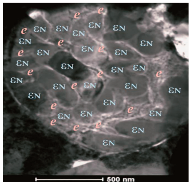
Fig. 22. The \varepsilon_N – sub-layer cross-section, ( \varepsilon_N – sub-layer is shown in Fig. 21, formerly named as the N – sub-layer, Fig. 13); some cells of the \varepsilon_N – phase are well visible; every cell is surrounded by the eutectic precipitate, e , in the micro scale (the phenomenon is identical to that revealed in the Fig. 9 and Fig. 11 in the macro scale)
