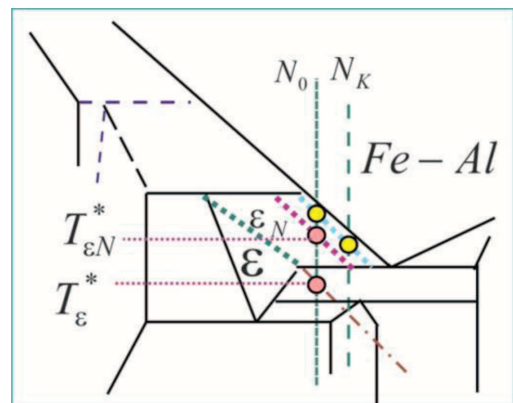
Fig. 18. Field for the appearance of the non-equilibrium \varepsilon_N – phase
